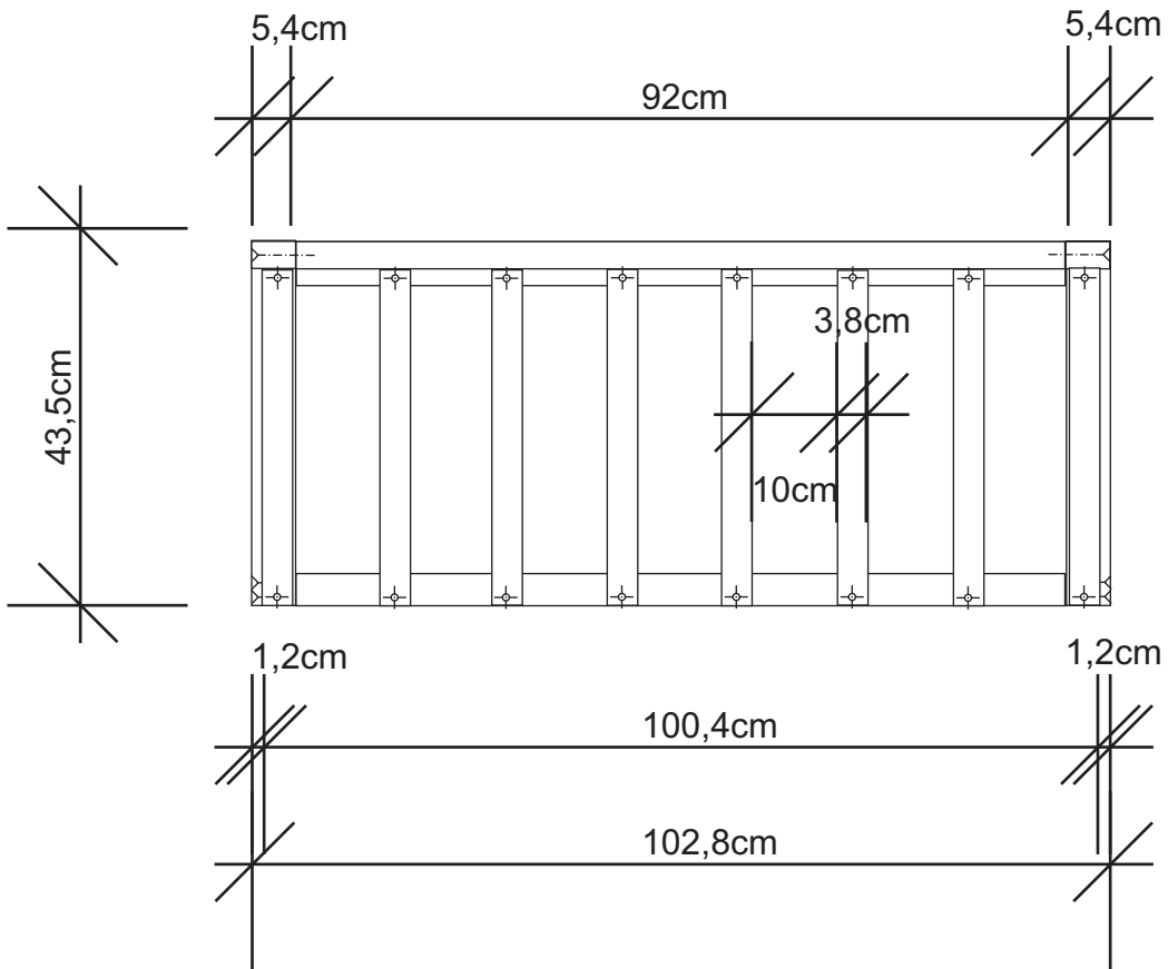
side view
